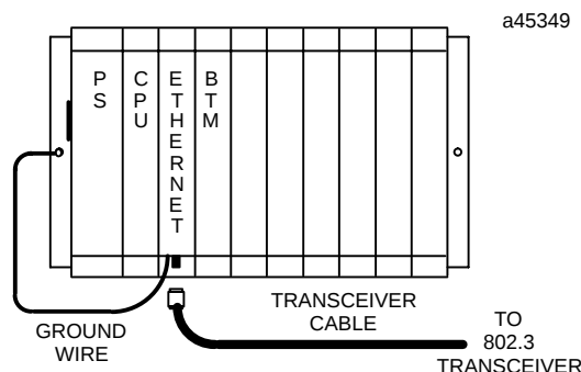
Figure 4. IC697 PLC Rack Layout
