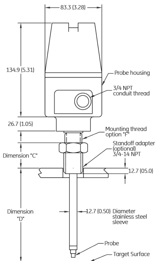
Figure 1: 21000/CA21000 Proximity Probe Housing Assembly
