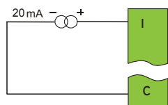
20mA Analog In - Self Powered
