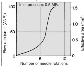
AS3201F, AS3211F AS3301F, AS3311F
