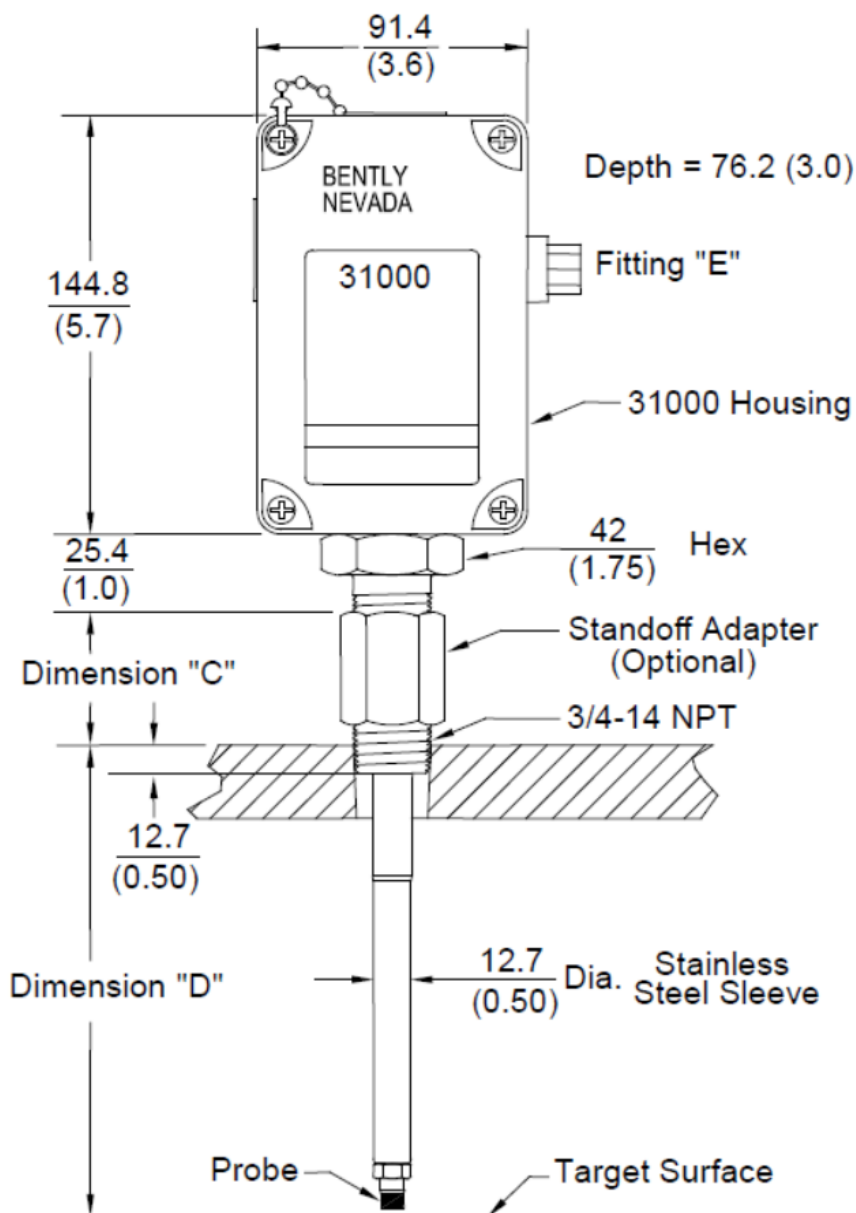
Figure 1: Dimensions for 31000 and 32000 Proximity Probe Housings
