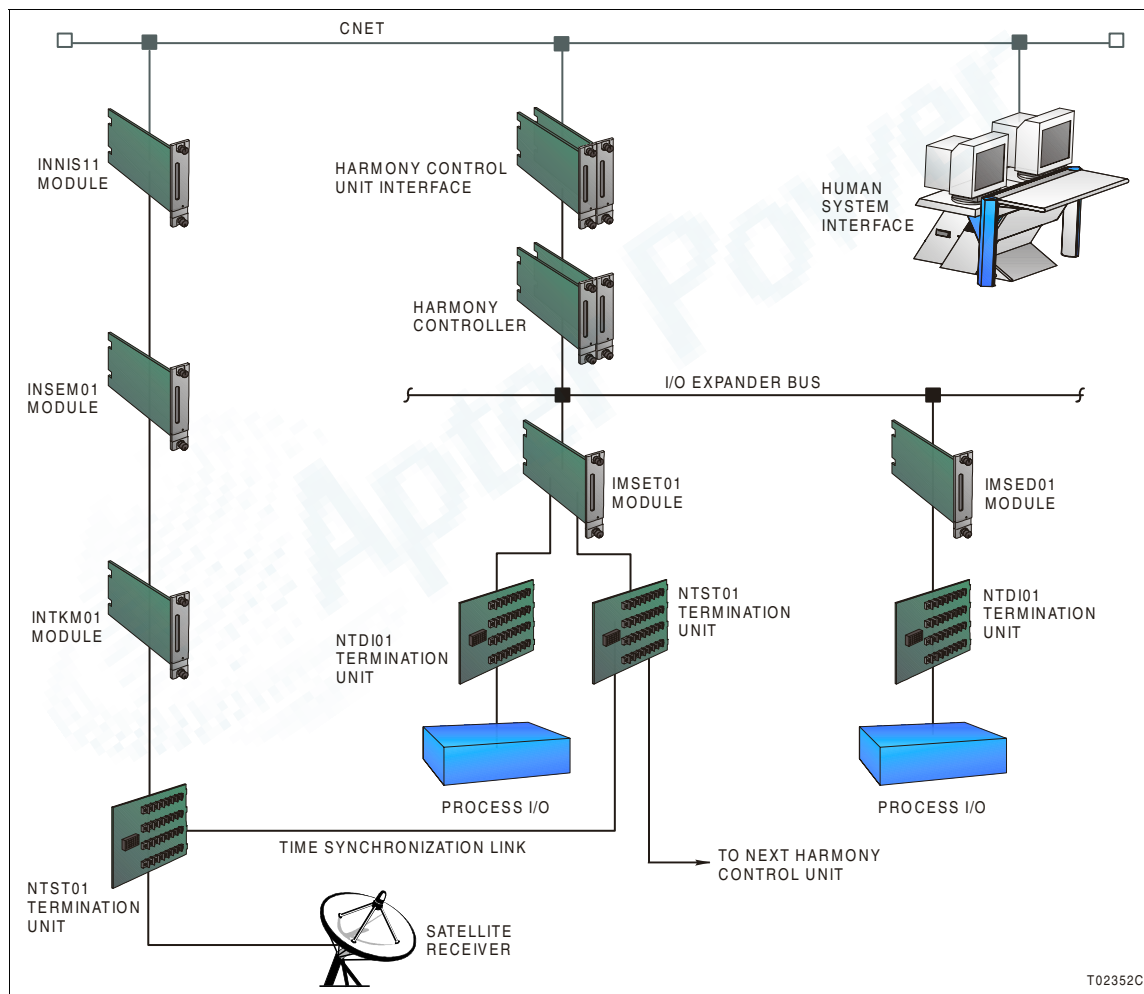
Figure 1. Distributed Sequence of Events System Architecture
