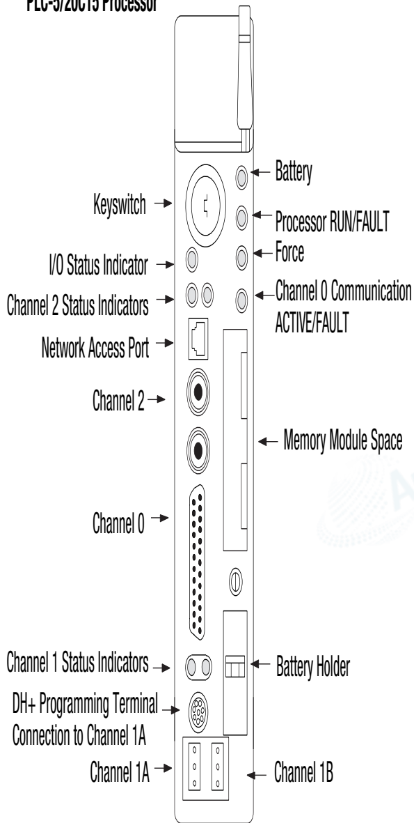
PLC-5/20C15 Processor
