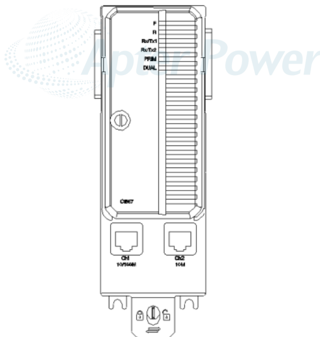
Figure 35. Modbus TCP Interface
